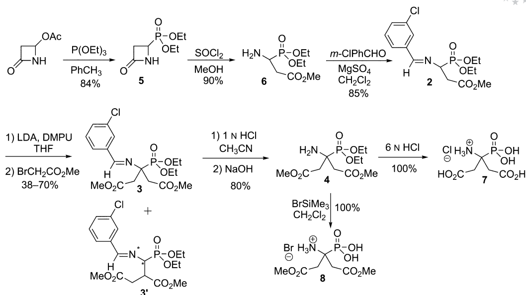
Scheme 2. Synthesis of target molecule 7.
