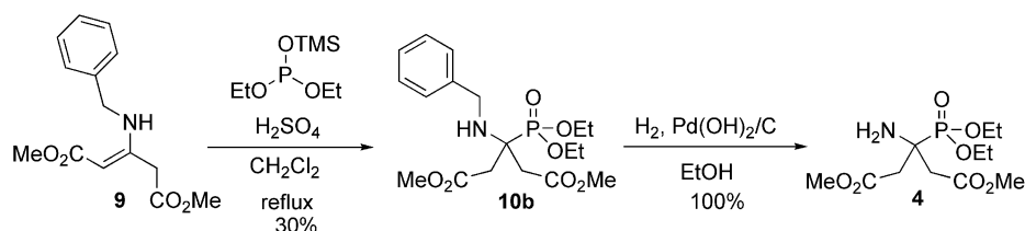
Scheme 4. Addition of diethyl trimethylsilyl phosphite to enamine 9 .
