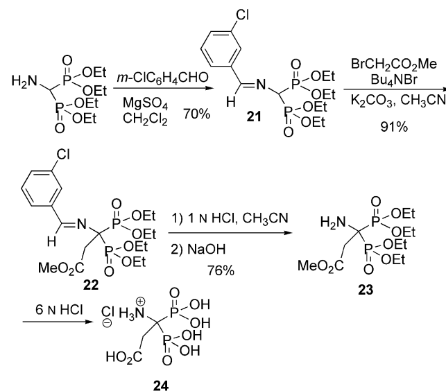
Scheme 7. Synthesis of \alpha -aminobis(phosphonic acid) 24 .
