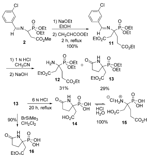
Scheme 5. Synthesis of compound 15 .
