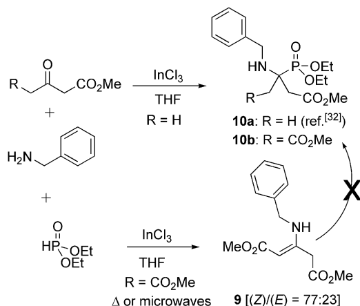
Scheme 3. Kabachnik–Fields reaction described by Ranu et al. ( 10a ) and applied to our substrate ( 10b ).
