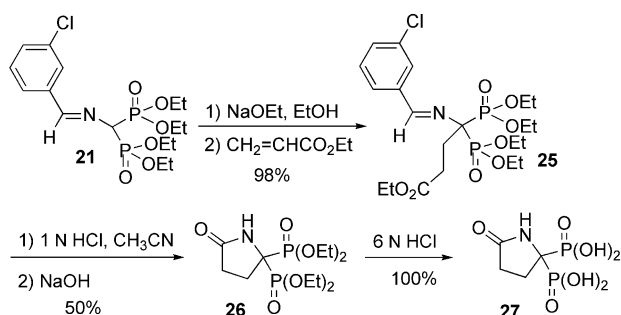
Scheme 8. Synthesis of pyrrolidinone 27 .
