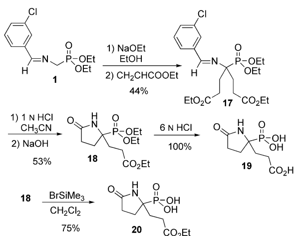
Scheme 6. Synthesis of compound 19 .
